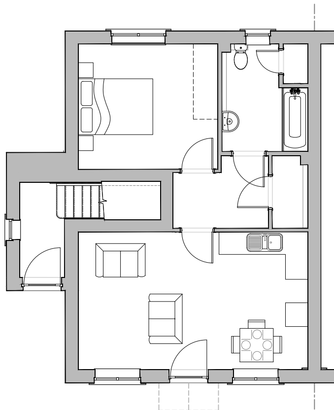
Ground Floor Layout (Approved Document M4(2) & NDSS Standards Compliant)
